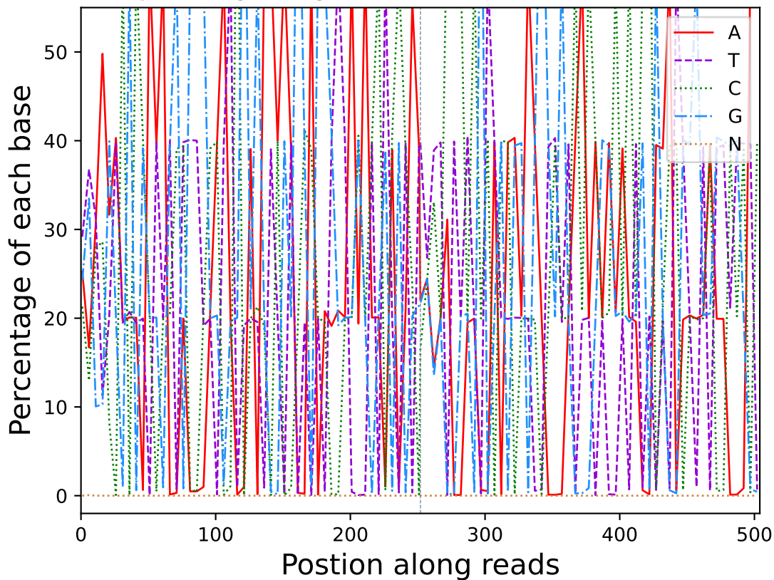
Base percentage along reads (R10617)
